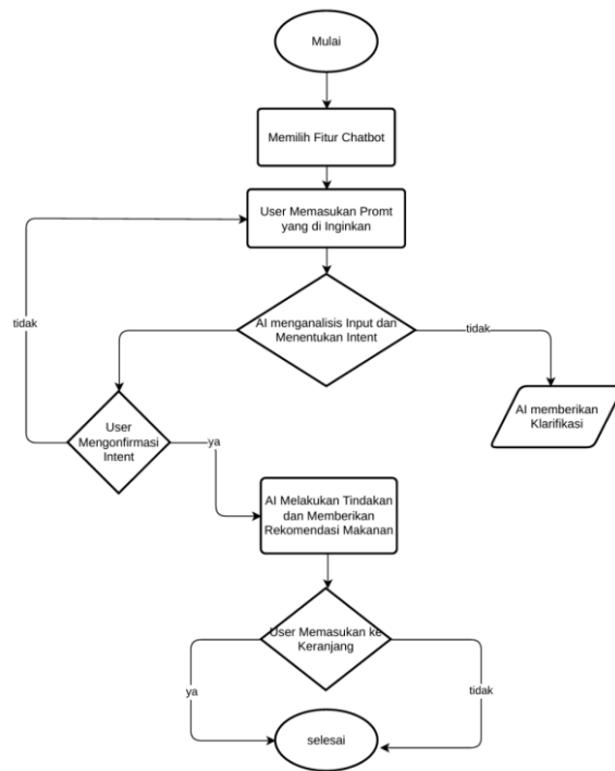
Flowchart 4. Flowchart fitur chatbot
